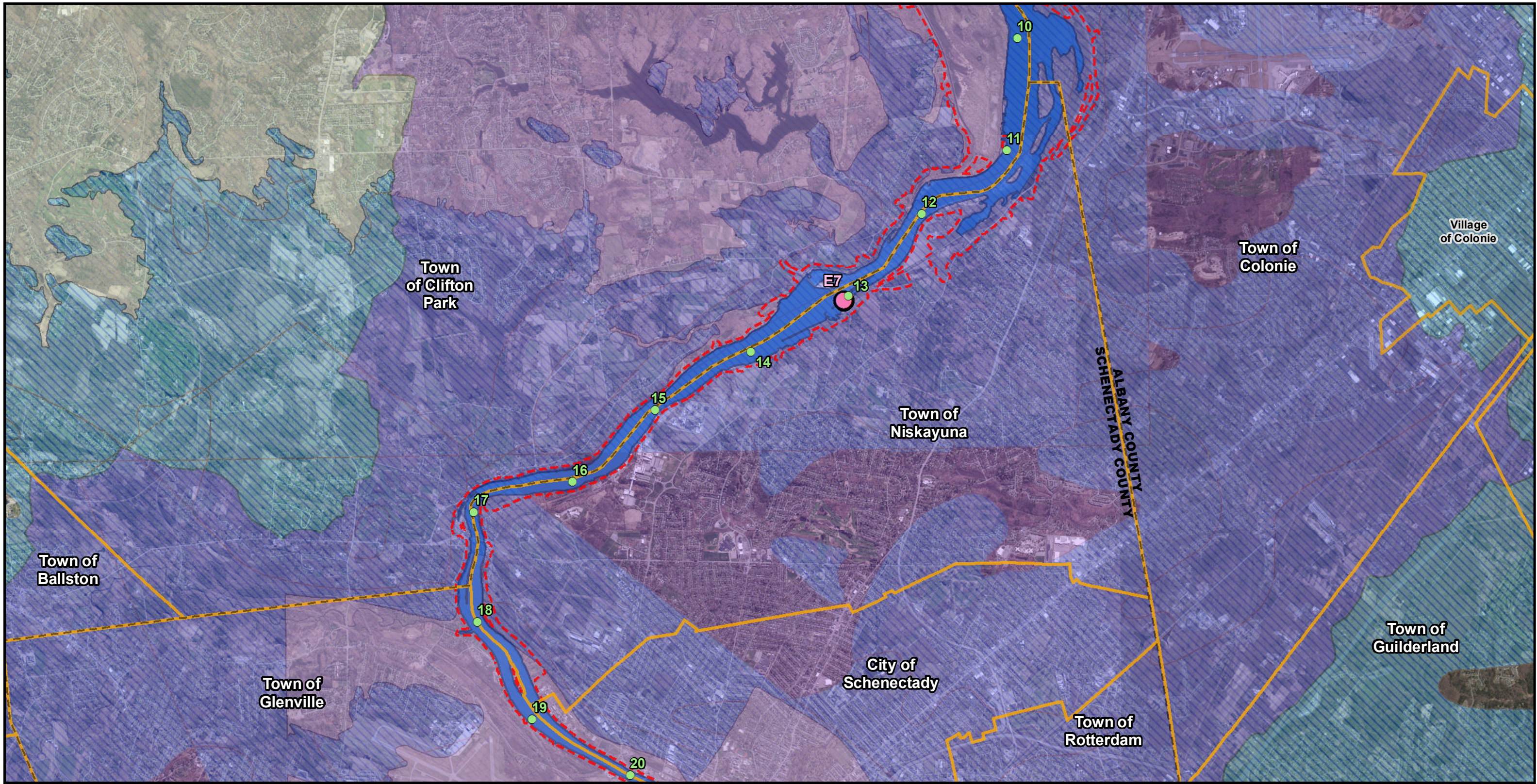
Figure 22F: Aquifers
